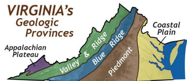
Source: William & Mary Geology Department
